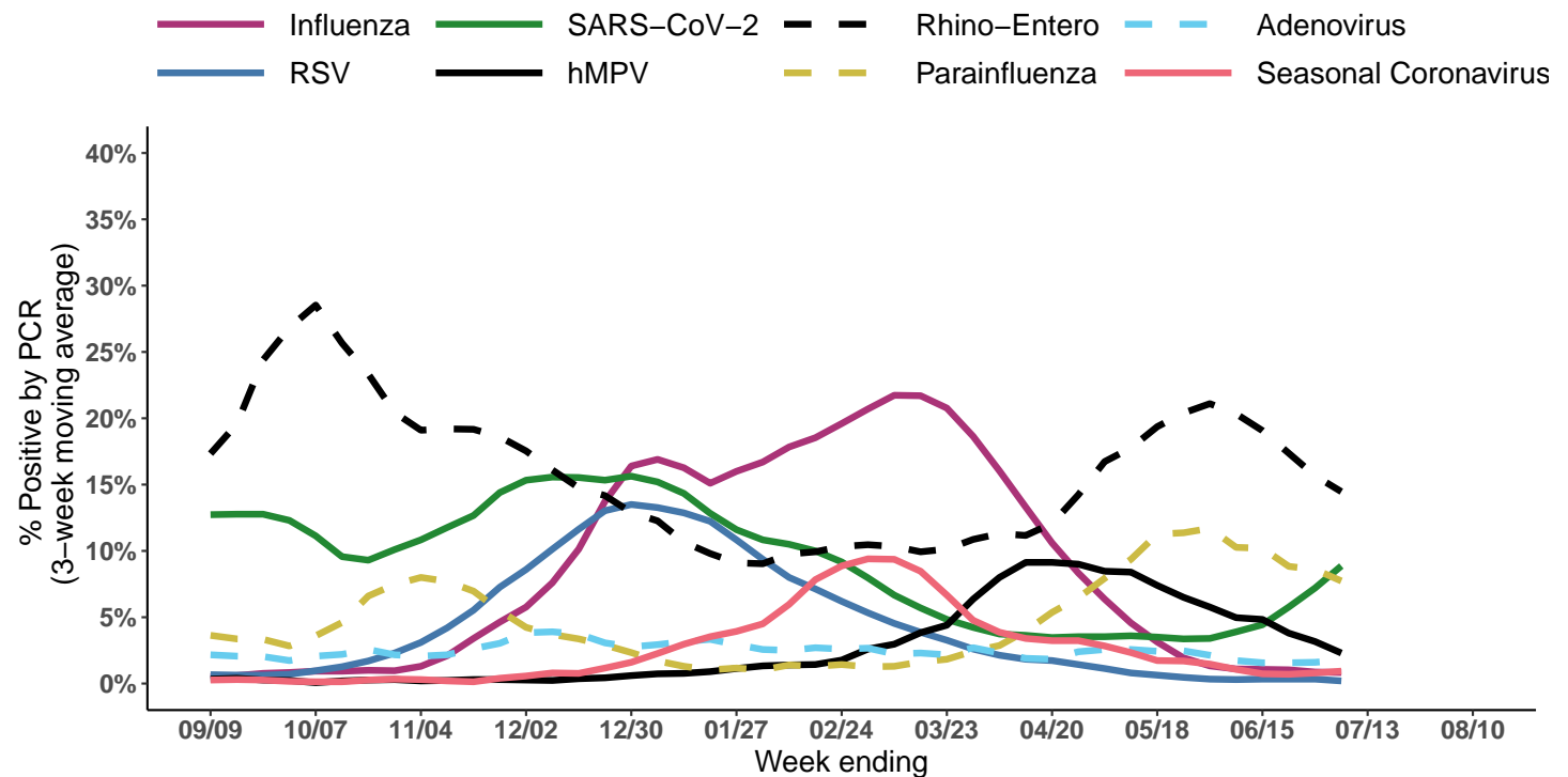
Number and percent positivity of respiratory viruses tested by PCR, NREVSS Week 27, Ending on July 06, 2024
