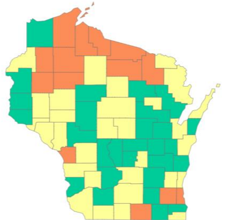
CDC COVID-19 Community Levels Updated: 7/15/2022
